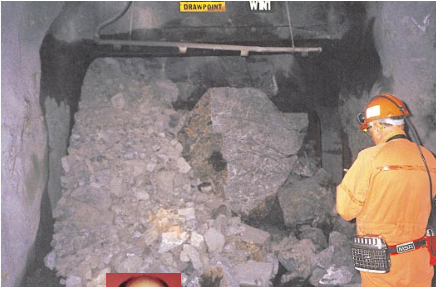
A large rock fragment in a drawpoint at the Northparkes mine, Australia
